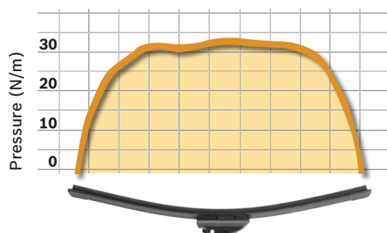
Beam windshield wiper
